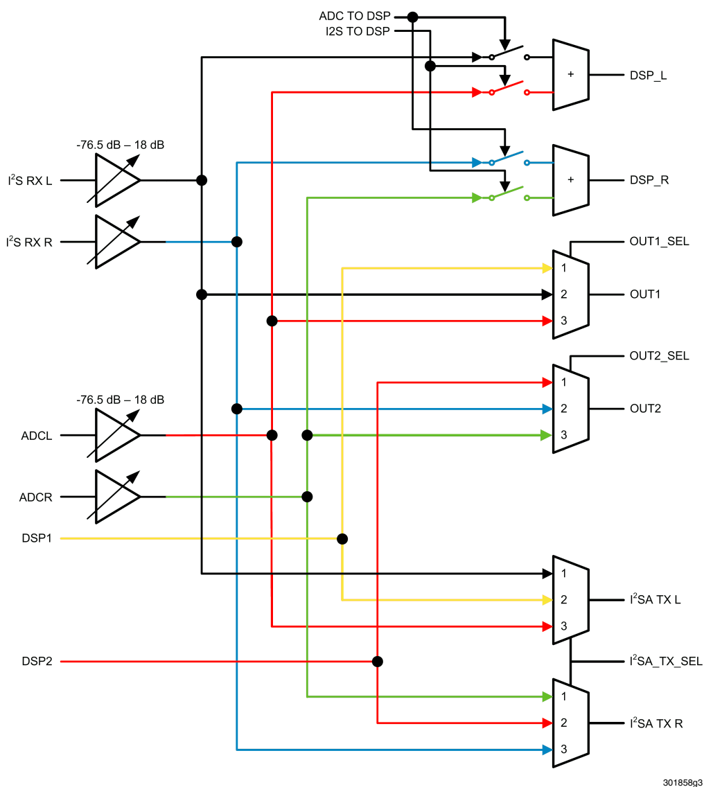
FIGURE 12. Digital Mixer
